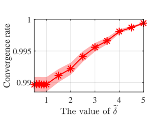
Figure 7: Convergence rate with different \hat{\delta} .
