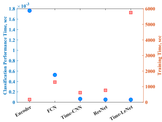
Fig. 11. Performance time. Online assessment and training
