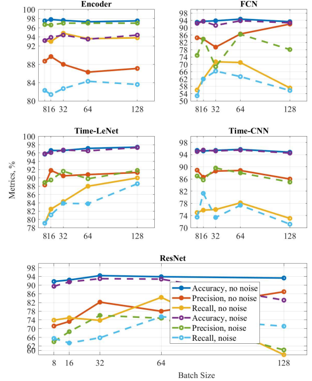
Fig. 7. Dependency on the batch size. Length=200 samples (3.33 sec)
