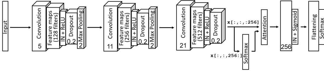
Fig. 5. Encoder neural network architecture
