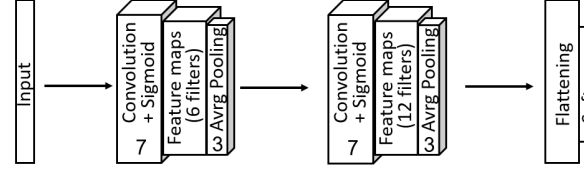
Fig. 4. Time-CNN neural network architecture
