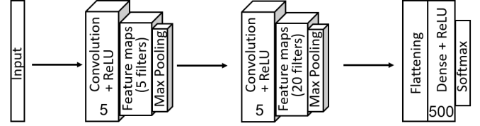
Fig. 3. Time-LeNet architecture
