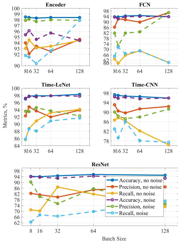
Fig. 8. Dependency on the batch size. Length=300 samples (5 sec)
