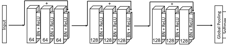
Fig. 6. ResNet neural network architecture
