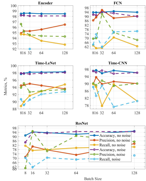
Fig. 9. Dependency on the batch size. Length=400 samples (6.67 sec)
