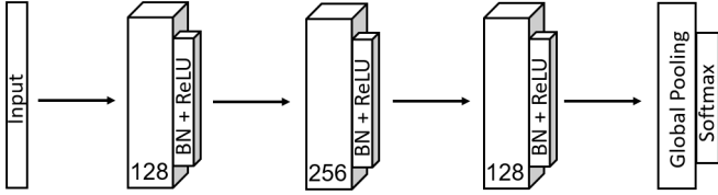
Fig. 2. Fully convolutional neural network architecture
