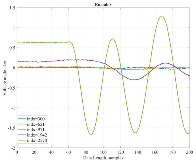
Fig. 12. Difference between missclassified data by Encoder and Time-LeNet. Batch = 64
