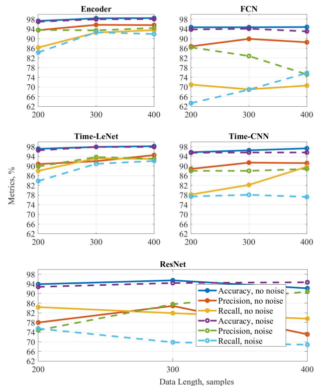
Fig. 10. Dependency of metrics on the length of data. Batch size=64. Accuracy of Prony method: for 200 samples - 80.54%, 300 samples - 88.99%, 400 samples - 92.69%
