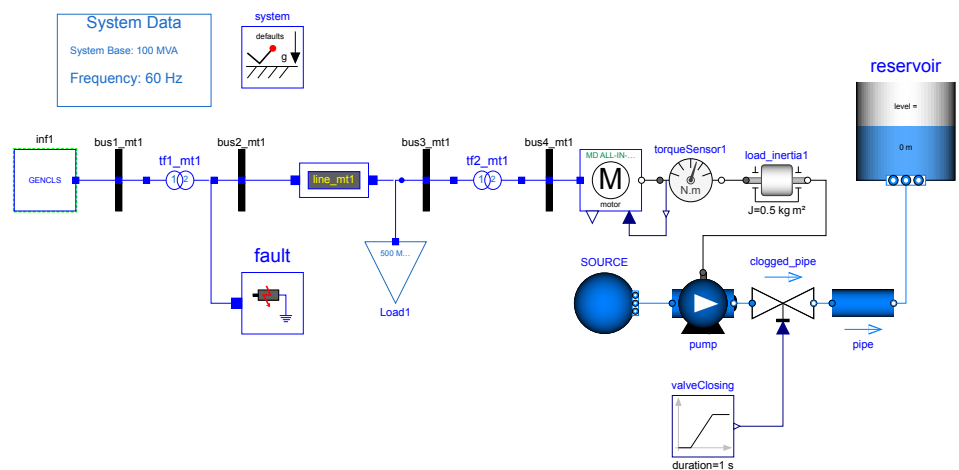
Figure 21. Multi-domain example that comprises OpenIPSL, newly developed components, and MSL Fluid components.
