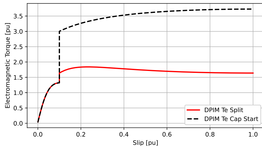
Figure 20. Electromagnetic torque versus slip for the split-phase and capacitor-start DPIM motor.
