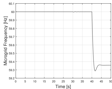
Figure 24. Simulation results: (a) microgrid active power import; (b) total active power consumption from the three non-multi-domain induction motors; (c) total active power consumption of the multi-domain motor; (d) water system mass flow rate; (e) microgrid frequency.
