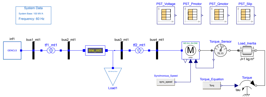
Figure 10. Multi-domain induction motor validation example.
