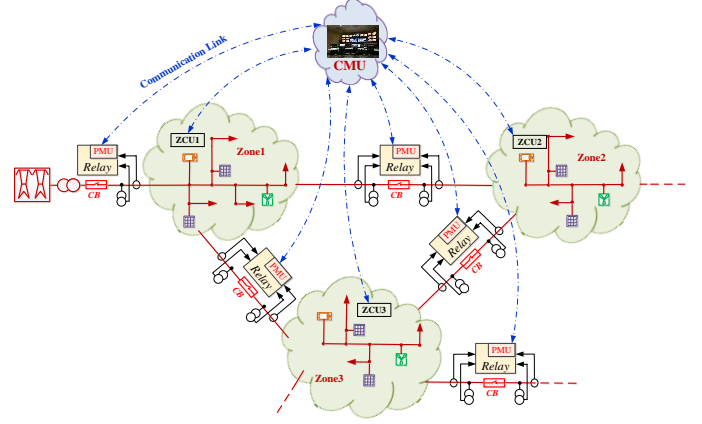
Fig. 1. Architecture required for the proposed NC method.
