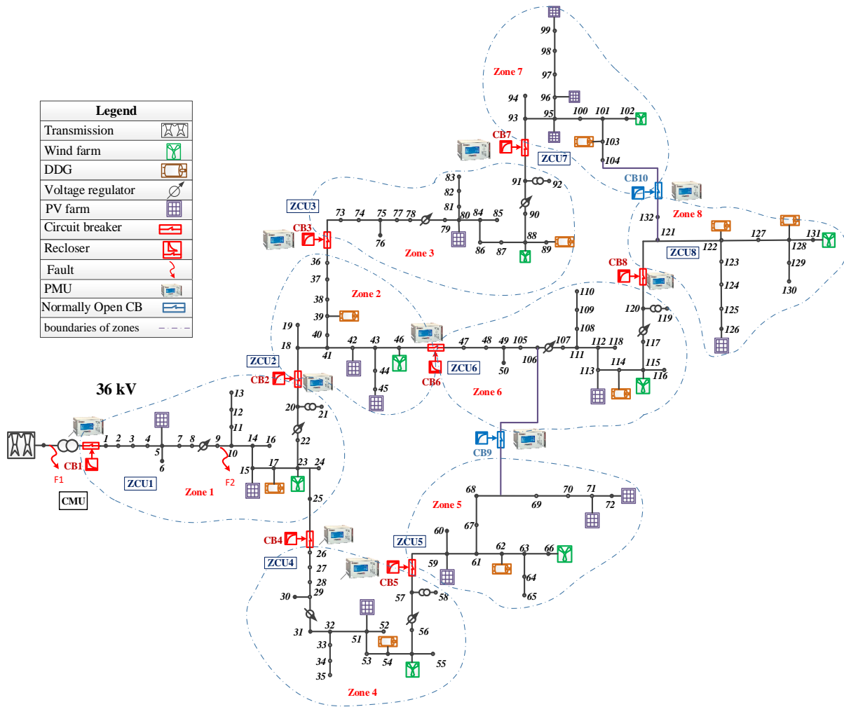
Fig. 4. The study distribution grid
