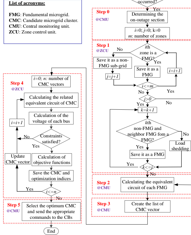
Fig. 3. The flowchart of the proposed NC method.
