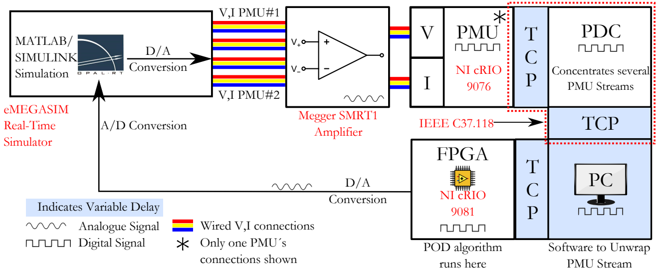
Fig. 4. Data path and experiment outling of HIL test. Hardware used is indicated in red text. Note that two PMUs are used though one is indicated. The section where synchrophasor data is used is indicated with a dotted line.
