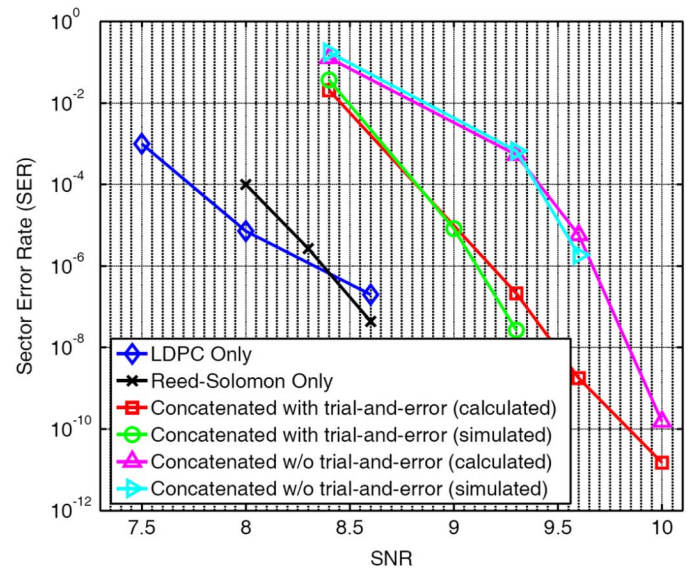
Fig. 3. SER performance comparison.
