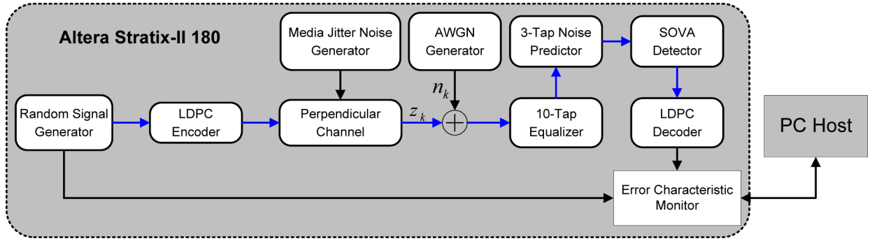
Fig. 1. FPGA-based simulation platform structure.
