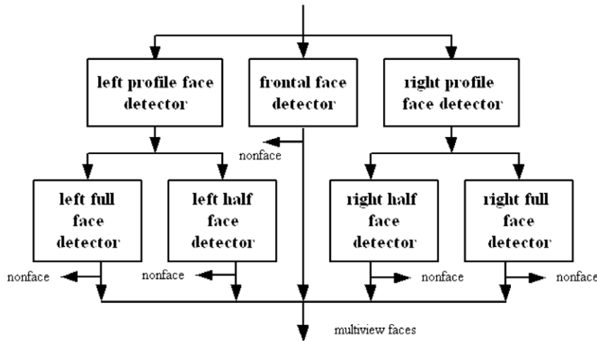
Fig. 10. The pyramid structure of multi-view face detector.
