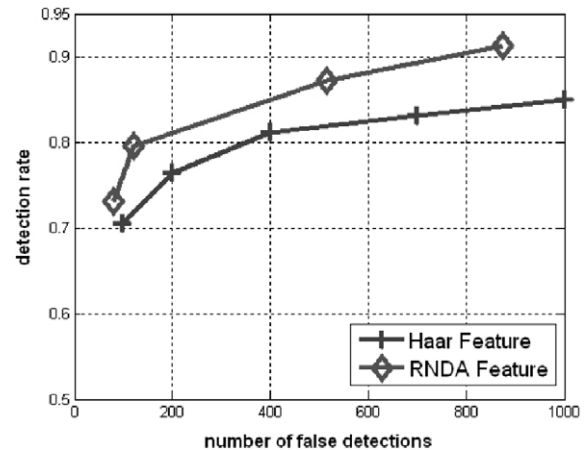
Fig. 11. ROC of profile face detection result on CMU test set. The results of Haar feature are from [12].
