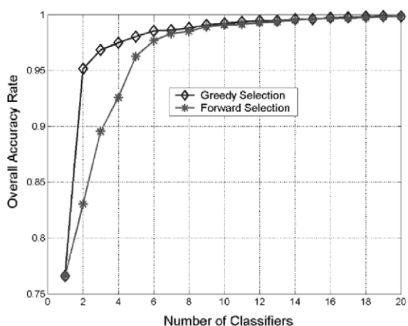
Fig. 6. Greedy training vs. forward selection.
