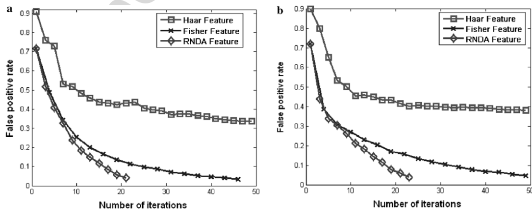
Fig. 5. Comparison of Haar features, Fisher features and RNDA features in AdaBoost. (a) Training results with half profile face data. (b) Training results with full profile face data.
