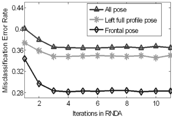
Fig. 3. Comparison of Fisher and recursive nonparametric discriminant analysis.
