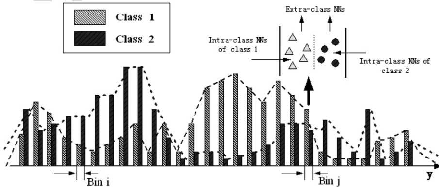
Fig. 2. Representing nearest neighbors using 1D feature histograms. Histograms of the face and non-face classes are calculated from the feature y = \Phi^T x . NNs are defined as the samples whose features are located in the same bin of the histograms.
