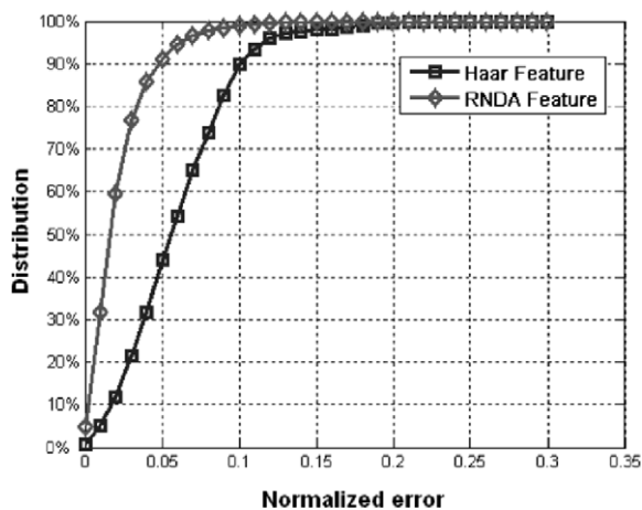
Fig. 14. Comparison of accumulated eye localization errors.
