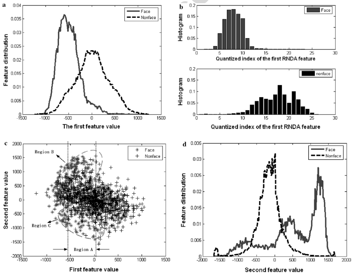
Fig. 4. Feature distribution on left full profile face data and non-face data. (a) Distribution of the first RNDA feature. (b) Histograms of the first RNDA feature. (c) Joint distribution of the first two RNDA features. (d) Distribution of the second RNDA feature.
