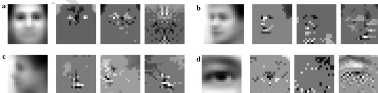
Fig. 9. Good features for multi-view face and eye detection. (a–c) The mean face and first three features for frontal faces, left half and left full profile faces respectively. (d) Mean eye and first three features for eyes.
