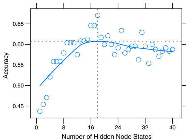
Fig. 3. The optimal number of hidden states was estimated by testing (cross validation within the training data) the accuracy of the HNB8 model across a range of hidden states. For 8 subjects, the HNB8 model performs best with 18 hidden states.
