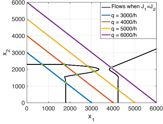
Fig. 7: Projection of the trip cost intersection in Fig. 6 on the x_1 - x_2 plane. Each trip rate corresponds to a single UE state indicated by the green points.
