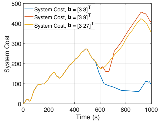
Fig. 12: System cost under different V2V bandwidth allocation policies. Bandwidth has the unit of Mbps, and is specified according to 802.11p protocol.
