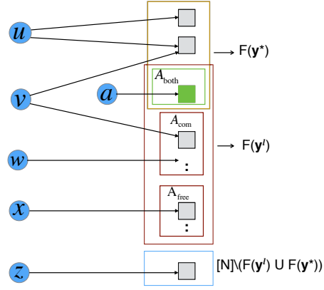
Fig. 2: As a consequence of Lemma 3, a given instance E gets transformed to a reduced instance E_1 which looks like above. Users whose demands do not get locally satisfied in either (\mathbf{y}^*, \mathbf{q}^*) or (\mathbf{y}^l, \mathbf{q}^l) in E look similar to z (Lemma 3(a)). Users whose demands get locally satisfied only in (\mathbf{y}^l, \mathbf{q}^l) look similar to either w or z (Lemma 3(b)). Users whose demands get locally satisfied only in (\mathbf{y}^*, \mathbf{q}^*) look similar to u (Lemma 3(c)). Users whose demands get locally satisfied in both (\mathbf{y}^*, \mathbf{q}^*) and (\mathbf{y}^l, \mathbf{q}^l) look similar to v or a (Lemma 3(d)).
