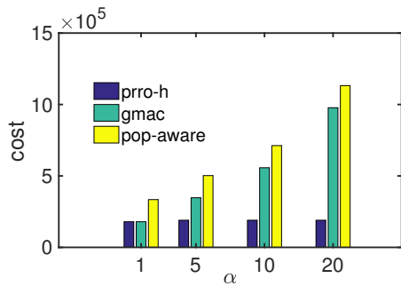
(a) linear storage cost with multicast server mode
