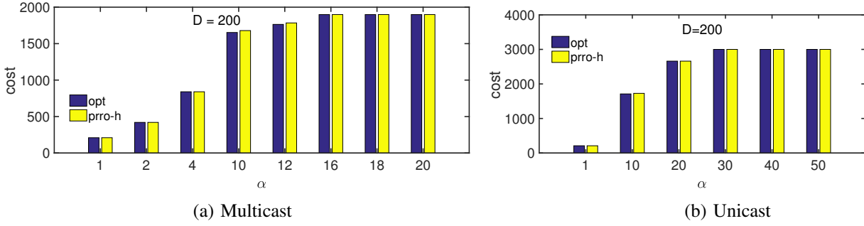
Fig. 4: Comparison of the cost of the output of LIN-GR (i.e., prro-h applied to MIP-a) with the cost of the optimal solution
