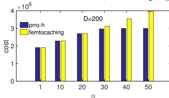
(c) linear storage cost with unicast server mode
