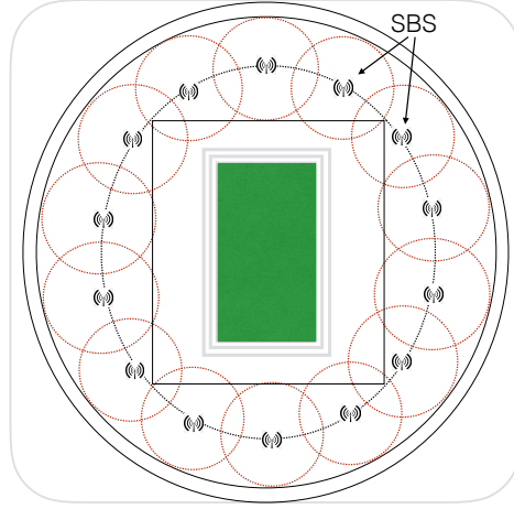
Fig. 3: Stadium consisting of 14 SBSs providing overlapping coverage to users. The requests that result in a cache miss at the SBS are served by a MBS (omitted here).
