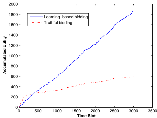
Fig. 2. The proposed learning-based bidding algorithm outperforms truthful bidding after the first 300 rounds.
