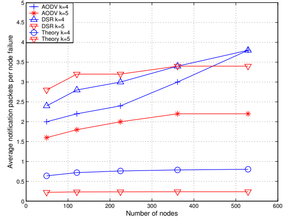
Figure 12: Average route error packets for a failed node as destination (46), c = 0.5 .
