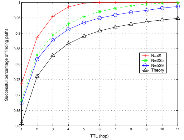
Figure 9: Successful percentage of finding paths as a function of TTL (10), k = 3 , c = 0.8 , AODV simulations.
